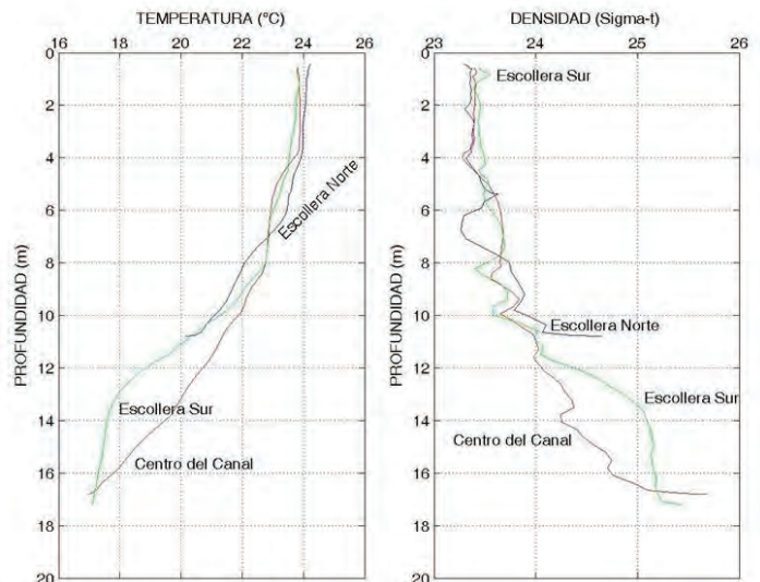
Data from a CastAway-CTD revealed to Rubèn Morales and his team from the Mexican Institute for Water Technology (IMTA) a strong temperature gradient at the mouth of Manzanillo harbor, directing further exploration of the harbor’s dynamics.
